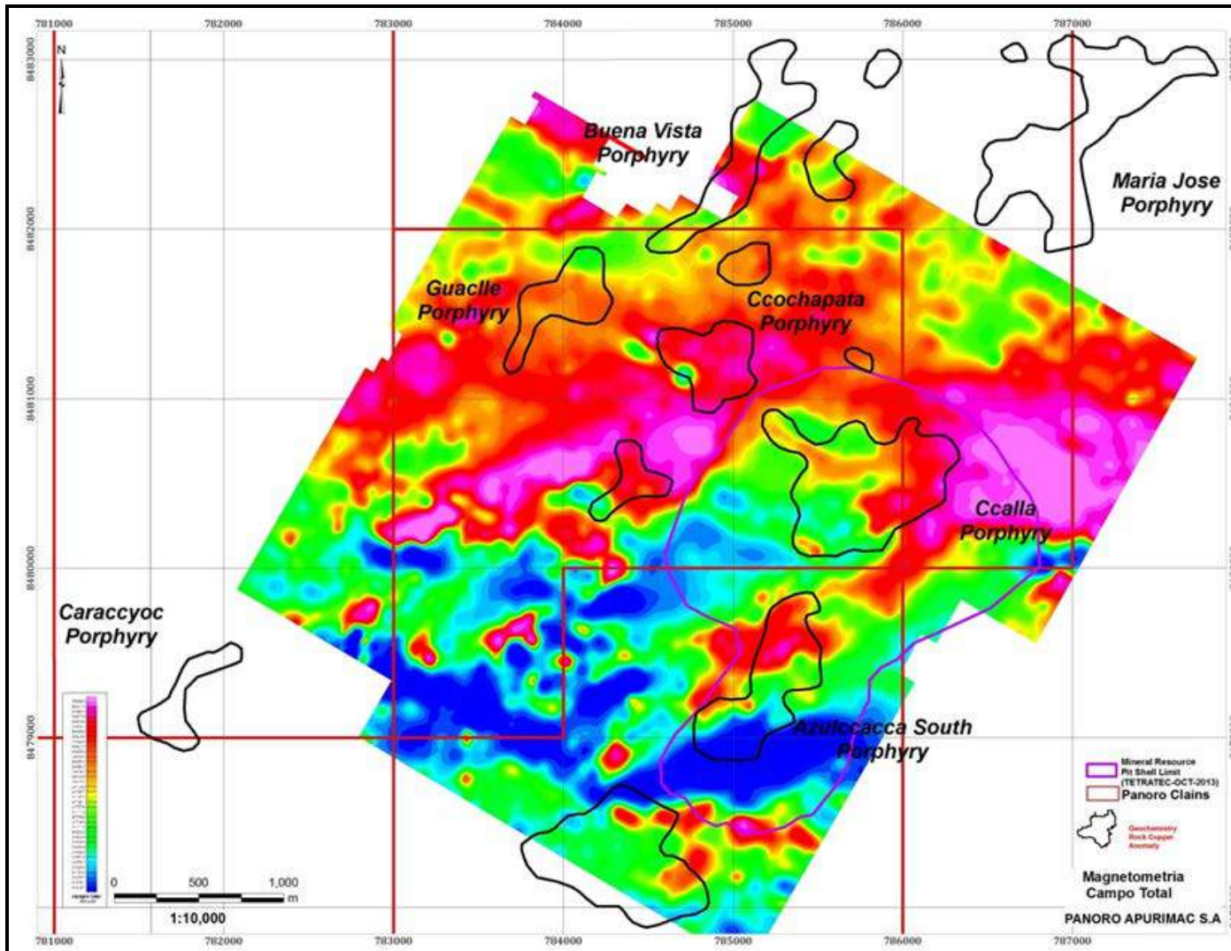
Figure 9.3 Total Field Magnetic Map
