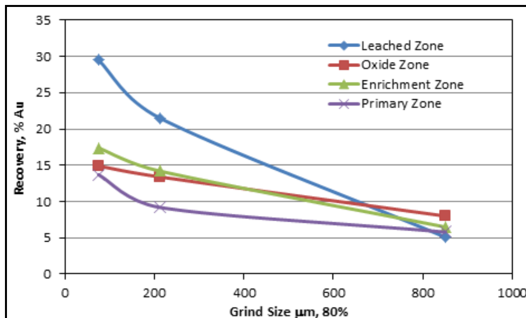
Figure 13.2 GRG Test Results
