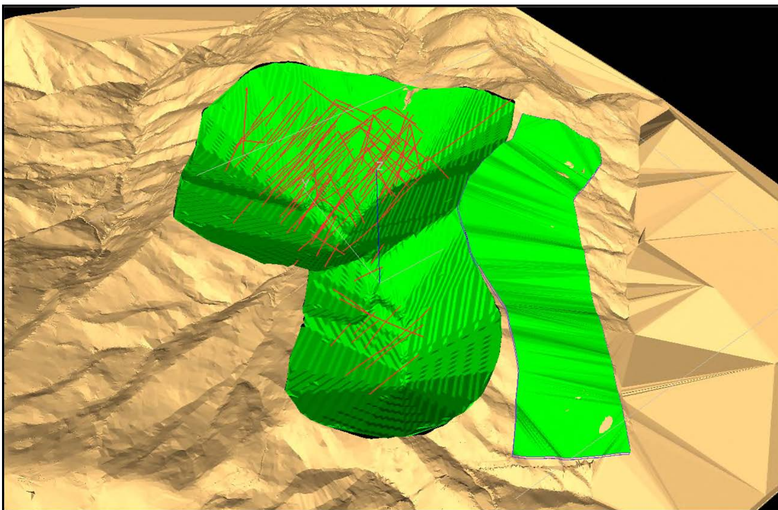
Figure 14.33 Isometric View of “Break-Even” Pit Looking to the Northeast with Exclusion Area of the Town of Cotabambas Shown in Green to the Southeast
