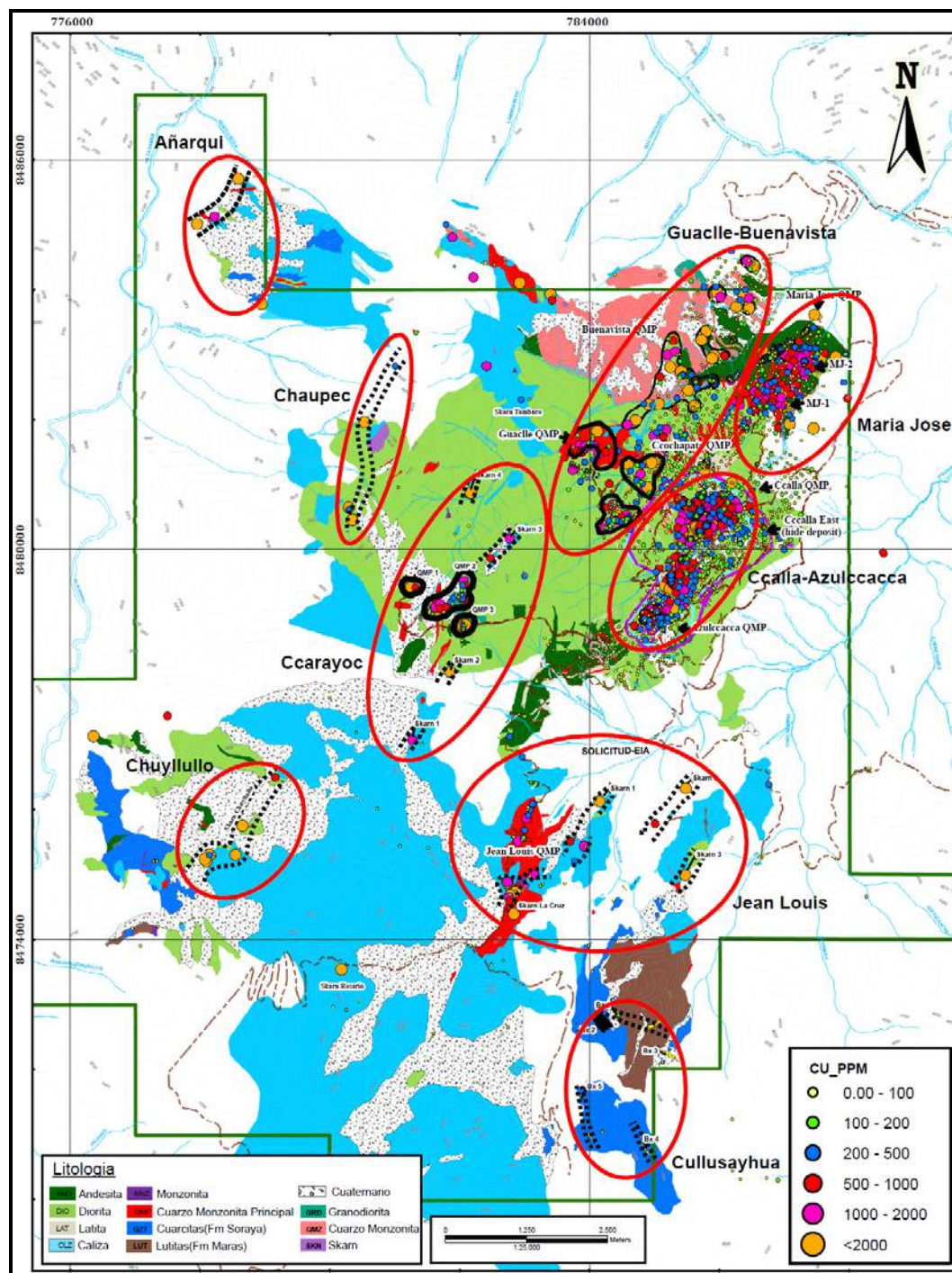
Figure 9.1 Exploration Targets on the Property
