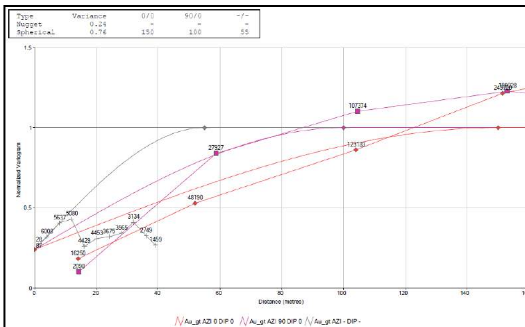
Figure 14.10 Gold Variograms for Zone 2 (Oxide Mineralization)
