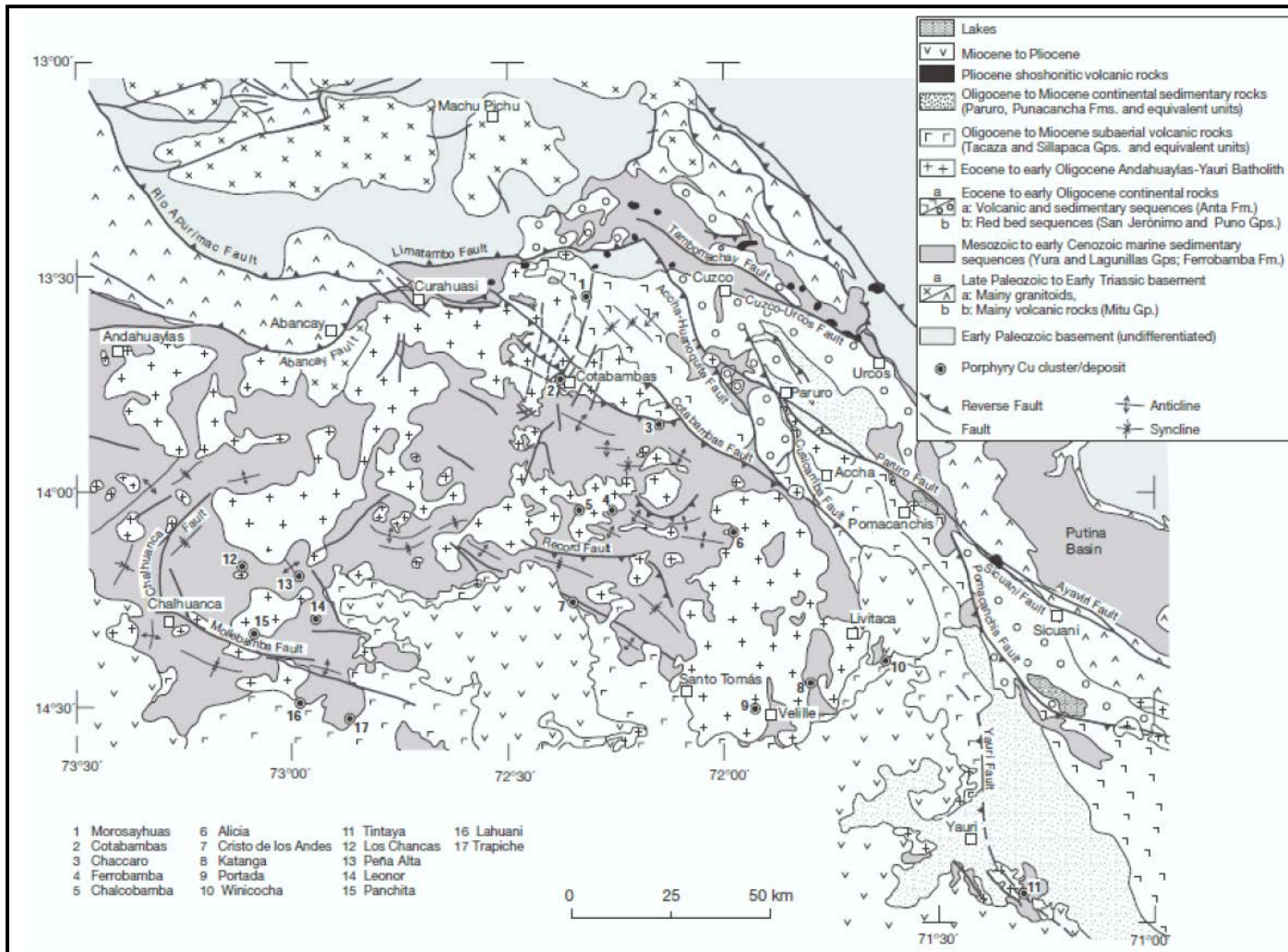
Figure 7.1 Regional Geology of the Yauli-Andahuaylas Belt
