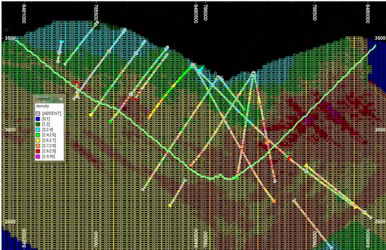
Figure 14.22 Density Northwest-Southeast Section Furthest to Northeast Showing Specific Gravity
