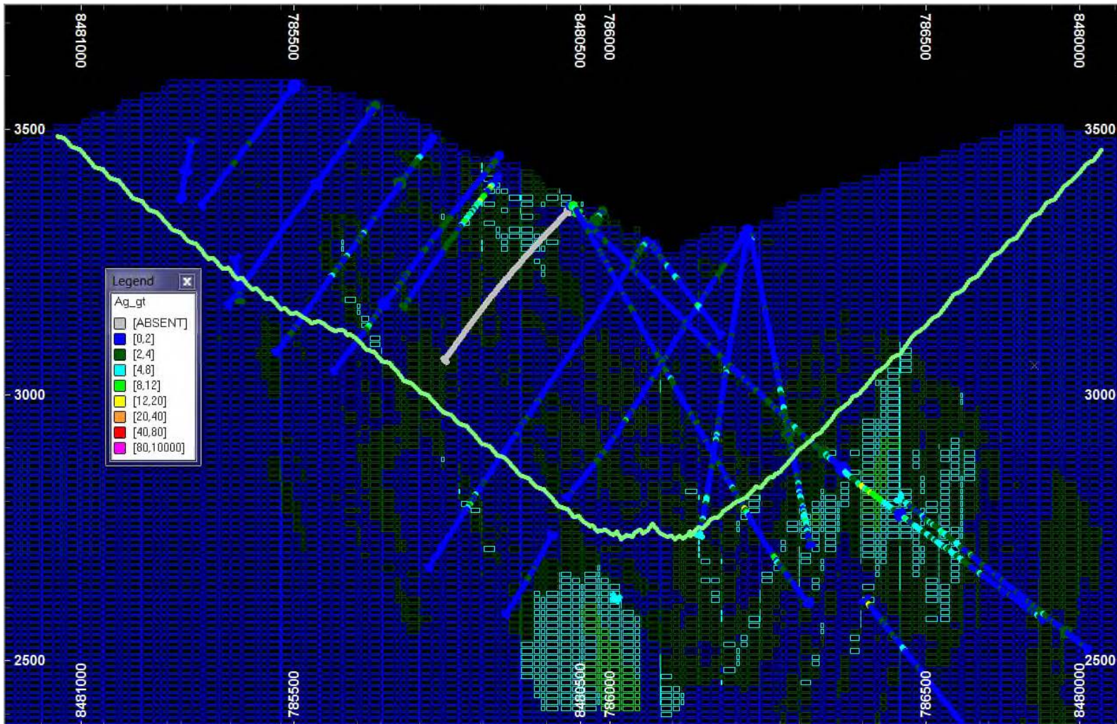
Figure 14.18 Silver Northwest-Southeast Section furthest to Northeast Showing Ag g/t
