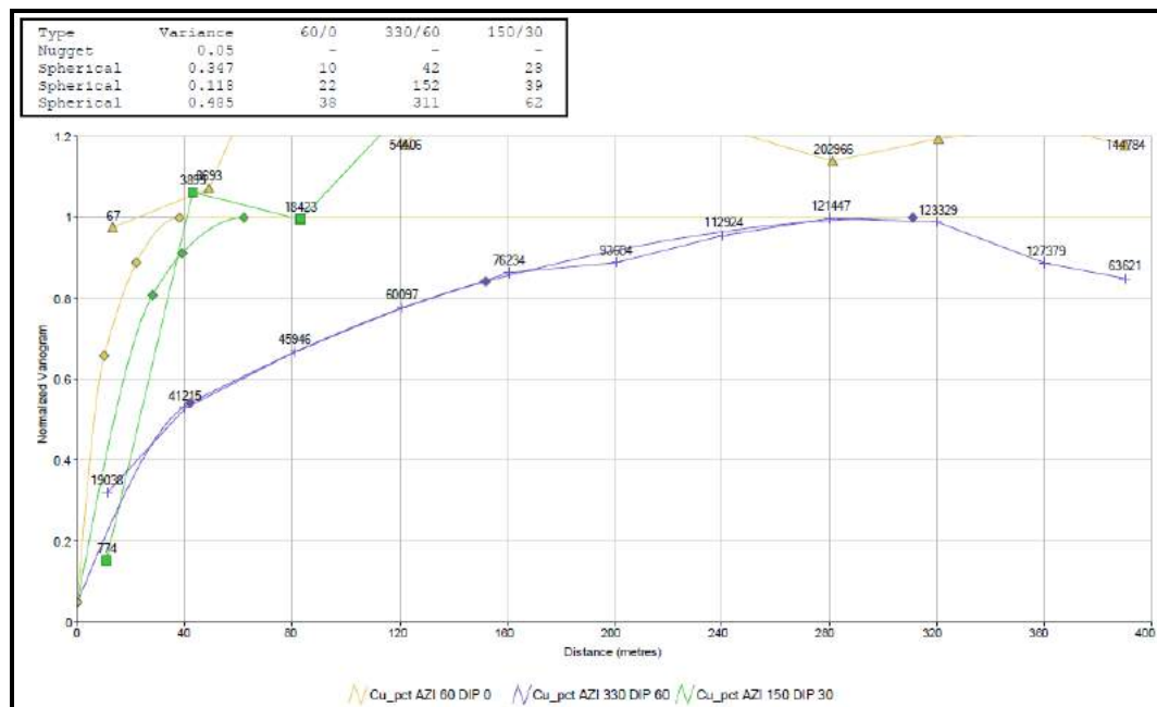
Figure 14.8 Copper Downhole Variograms for Zone 1 (Hypogene Mineralization)
