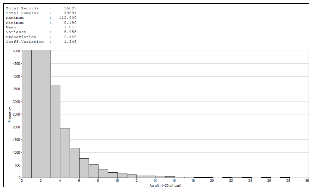
Figure 14.5 Silver Log Histogram of Raw Drillhole Data
