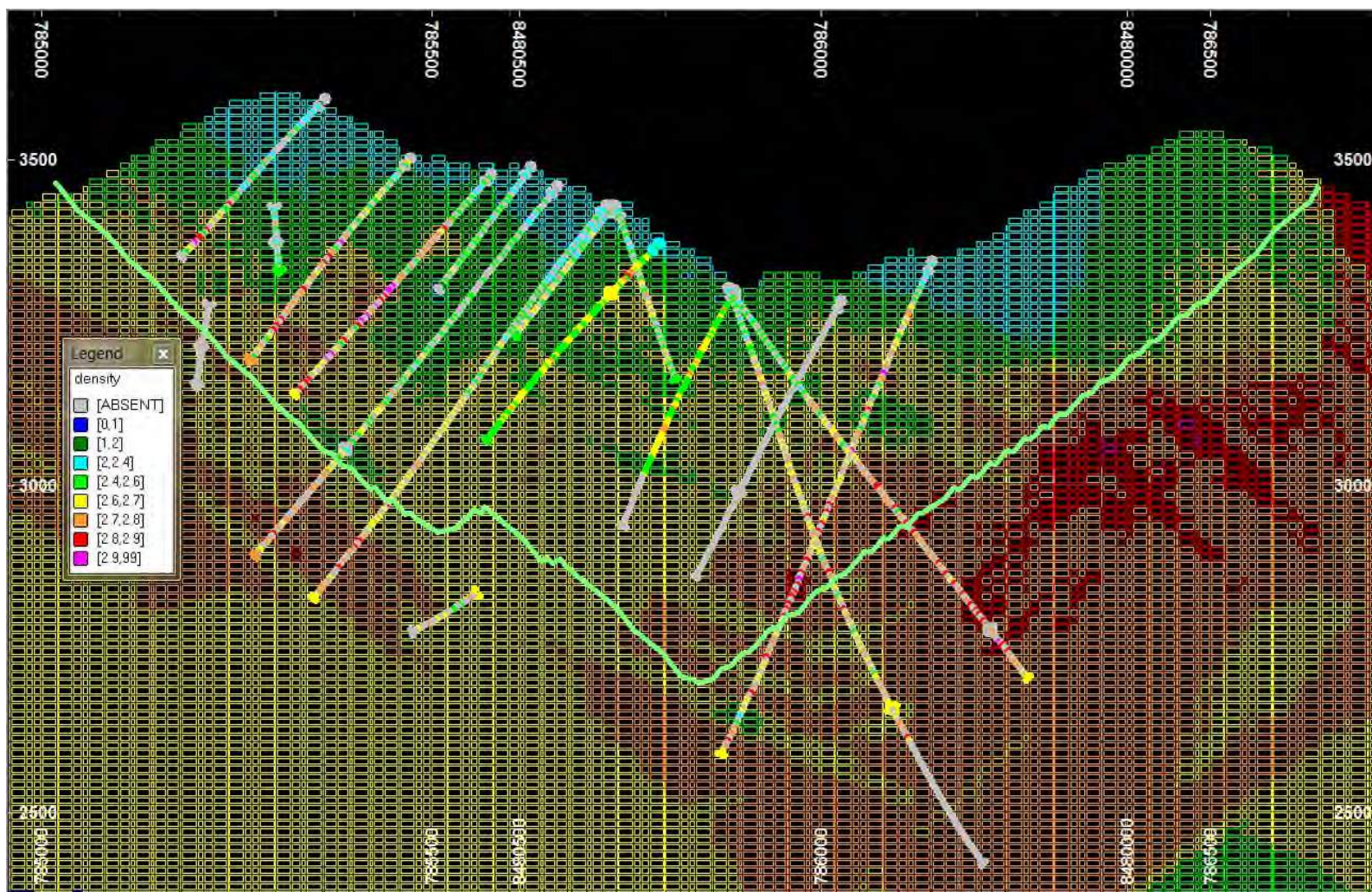
Figure 14.23 Density Northwest-Southeast Section Furthest to Northeast Showing Specific Gravity
