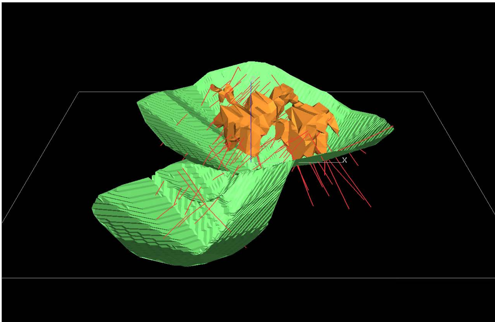
Figure 14.31 Resource Indicated Classification Wireframe within Conceptual Pit Shell
