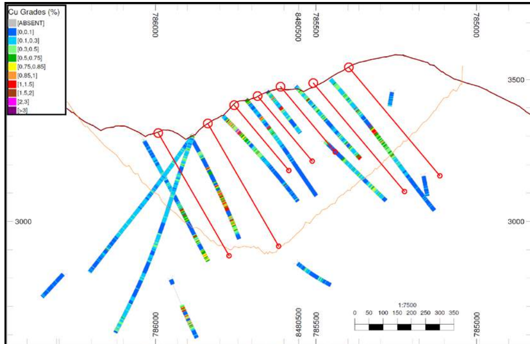
Figure 18.2 Proposed Infill Drilling Program – Representative Section View
