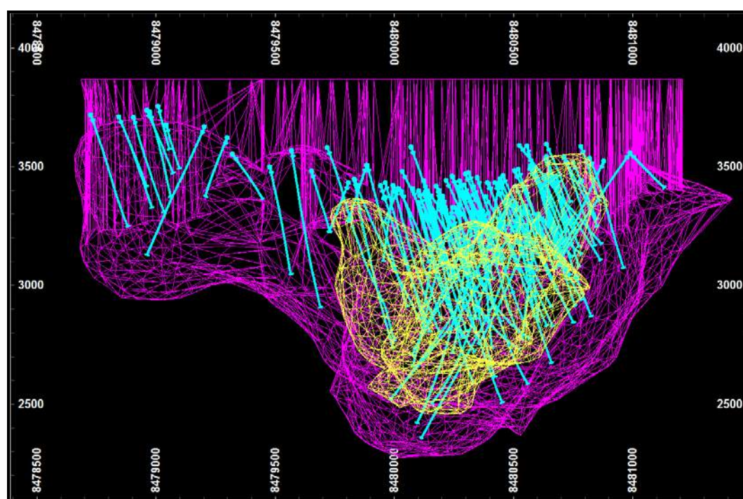
Figure 14.2 West-east Cross-section of Data Wireframes (magenta for copper, gold and silver; yellow for molybdenum)
