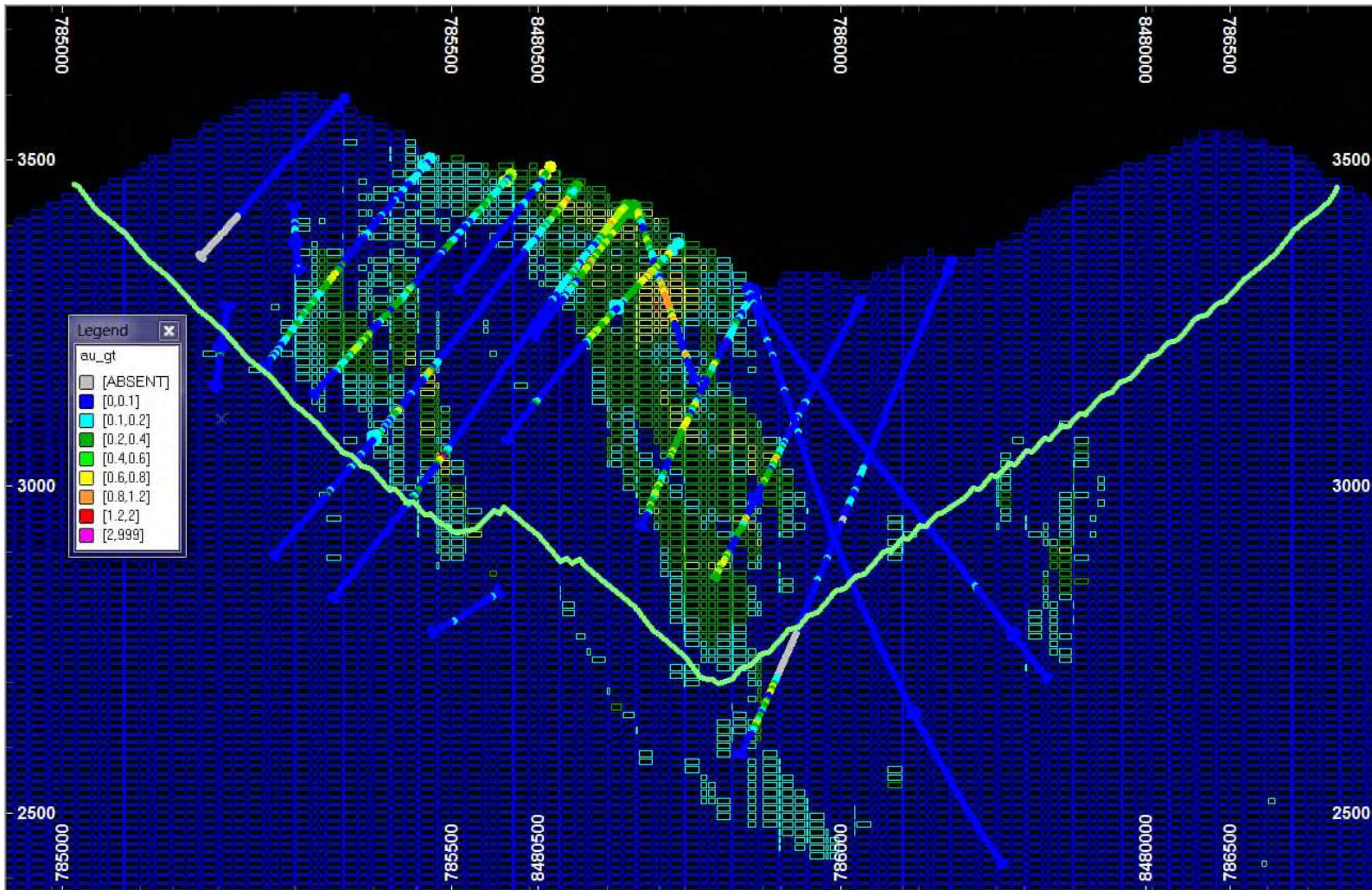
Figure 14.17 Gold Northwest-Southeast Section Furthest to Southwest Showing Au g/t
