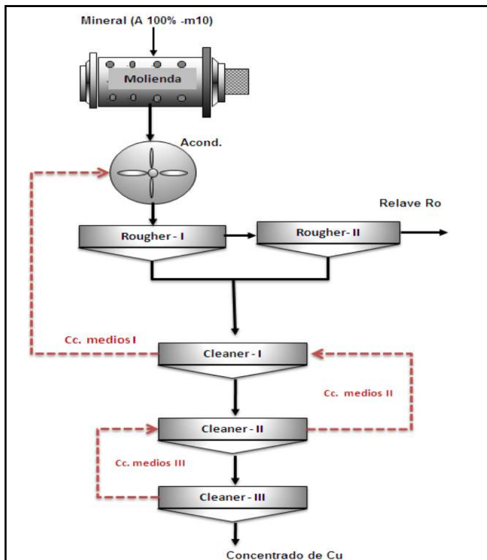
Figure 13.1 Hypogene Sulphide Locked Cycle Flotation Flowsheet
