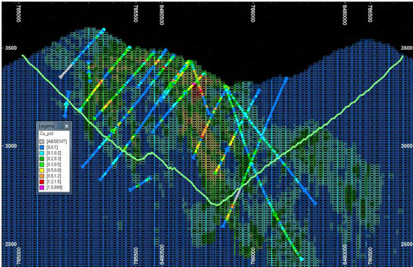
Figure 14.15 Copper Northwest-Southeast Section Furthest to Southeast Showing Cu %
