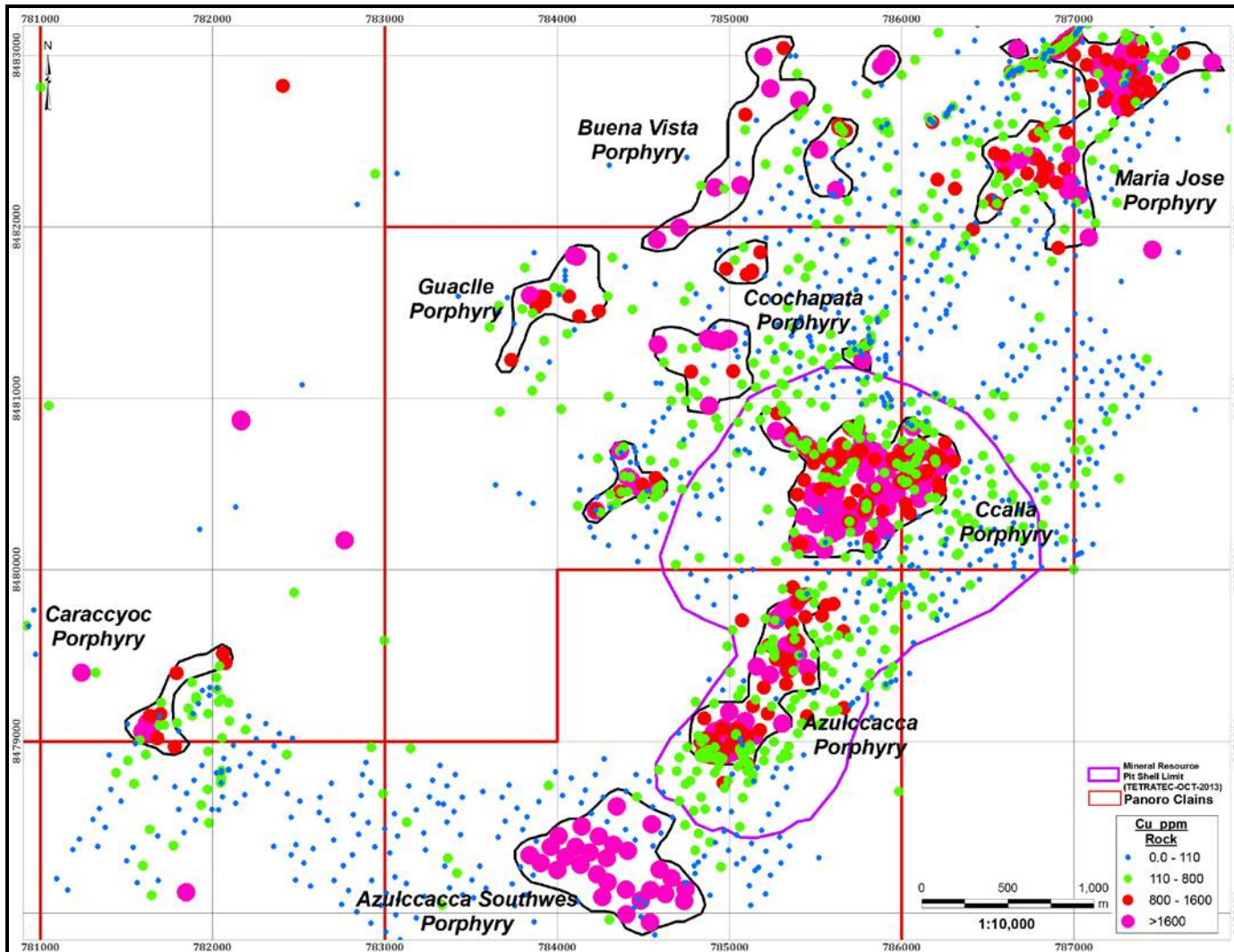
Figure 9.2 Rock Geochemical Map of Copper
