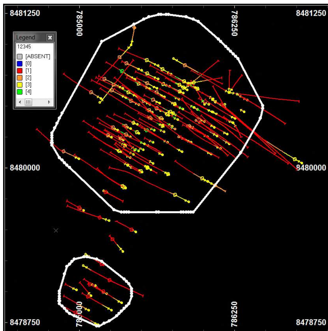
Figure 10.1 Drillhole Location Map
