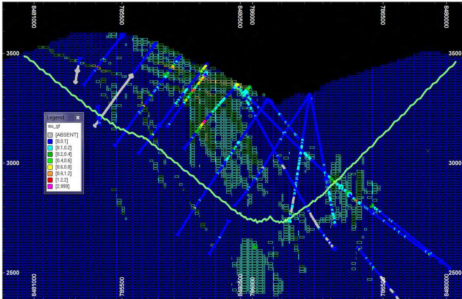
Figure 14.16 Gold Northwest-Southeast Section Furthest to Northeast Showing Au g/t
