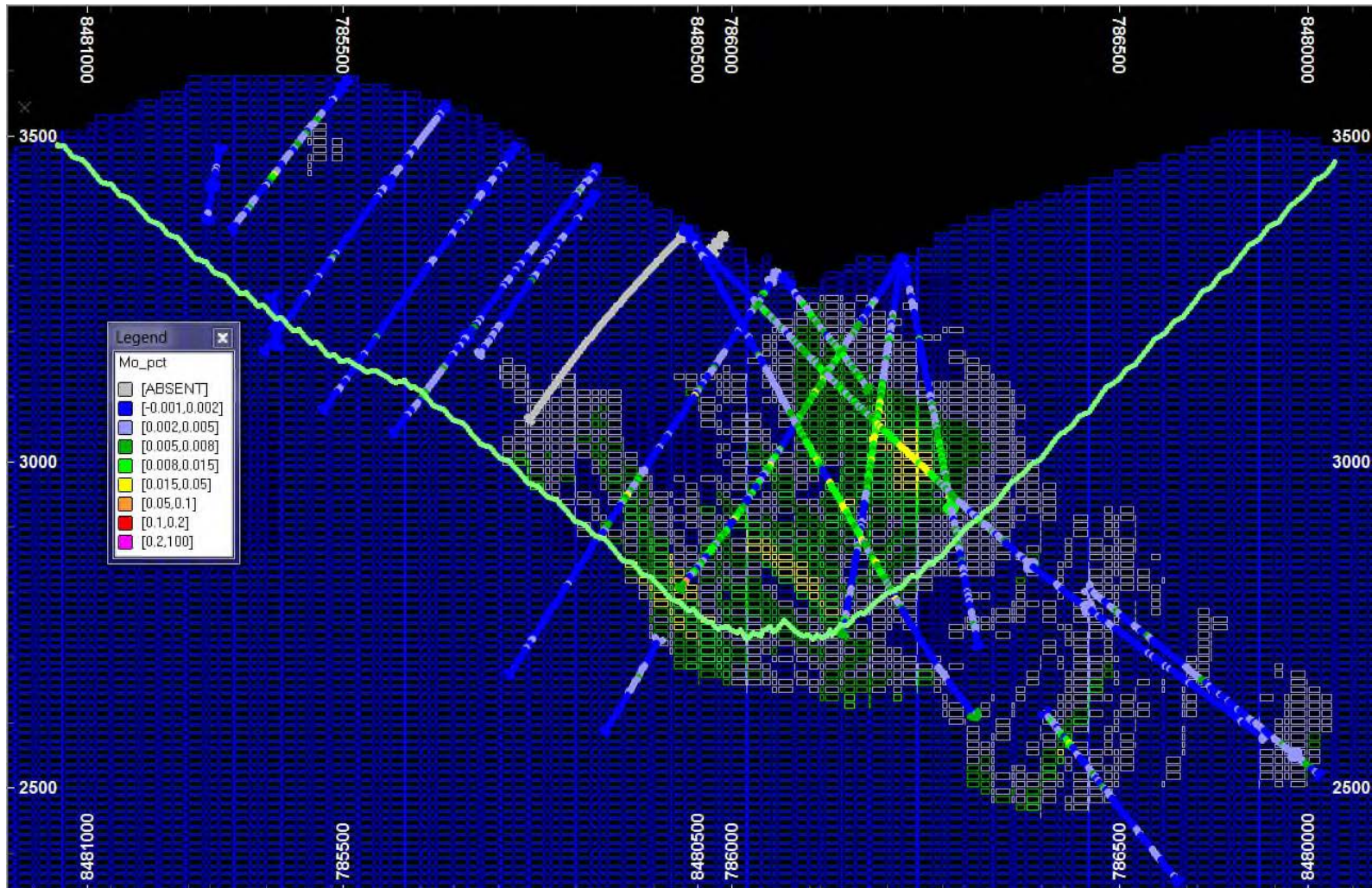
Figure 14.20 Molybdenum Northwest-Southeast Section Furthest to Northeast Showing Mo %
