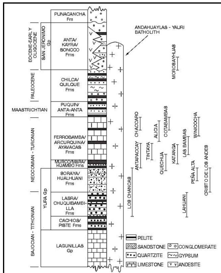
Figure 7.2 Regional Stratigraphy for the Cotabambas and Other Deposits
