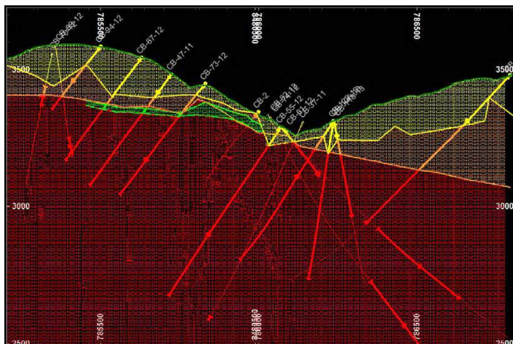
Figure 14.12 Northwest-southeast Cross-section of Domain Wireframes with Drillhole Traces and Block Model, Coloured by Domain (yellow – leached cap, orange – oxide, bright green – supergene, red – hypogene)
