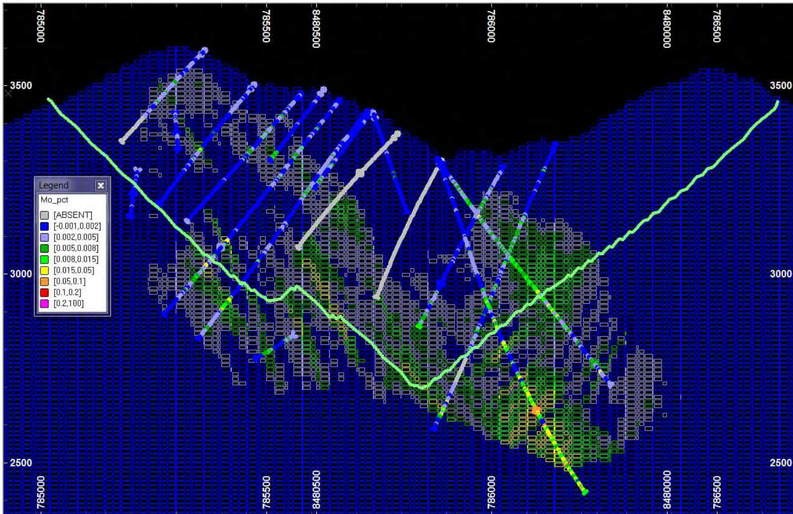
Figure 14.21 Molybdenum Northwest-Southeast Section Furthest to Southwest Showing Mo %
