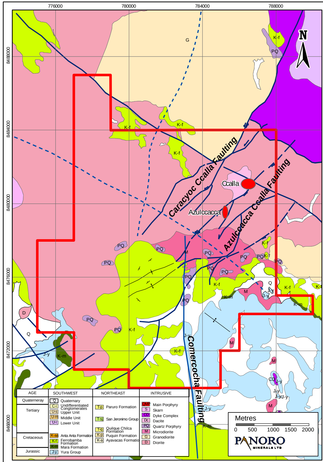
Figure 7.3 Geology of the Cotabambas Property
