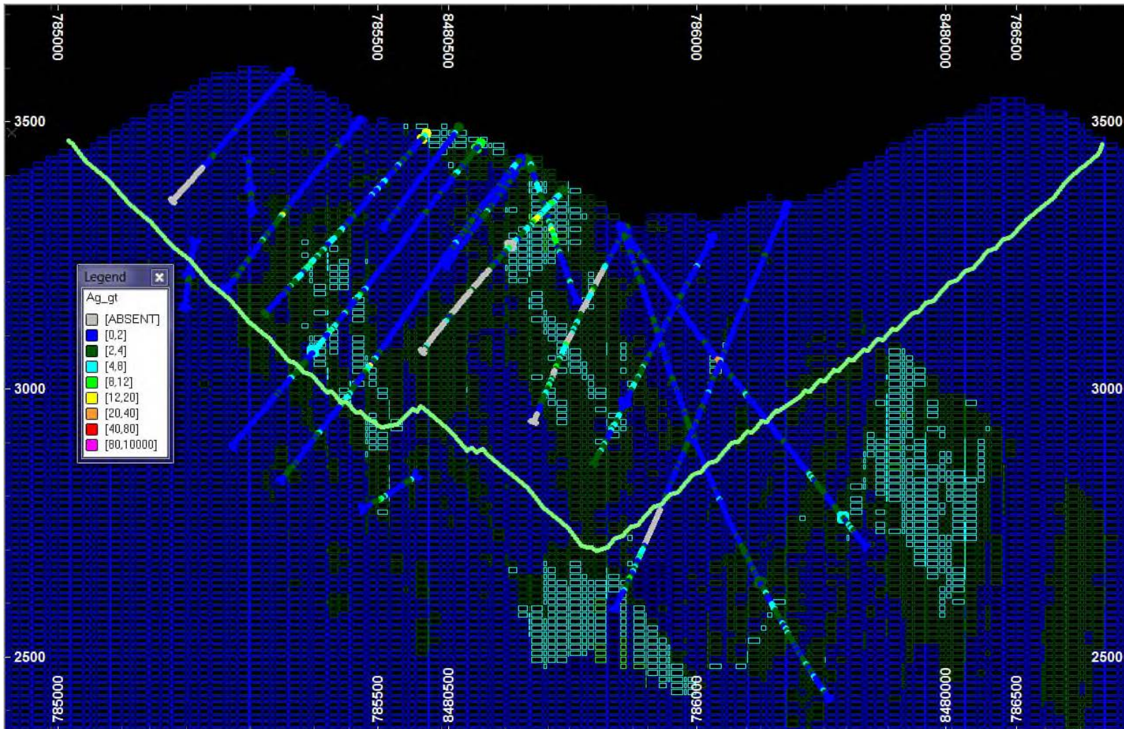
Figure 14.19 Silver Northwest-Southeast Section Furthest to Southwest Showing Ag g/t
