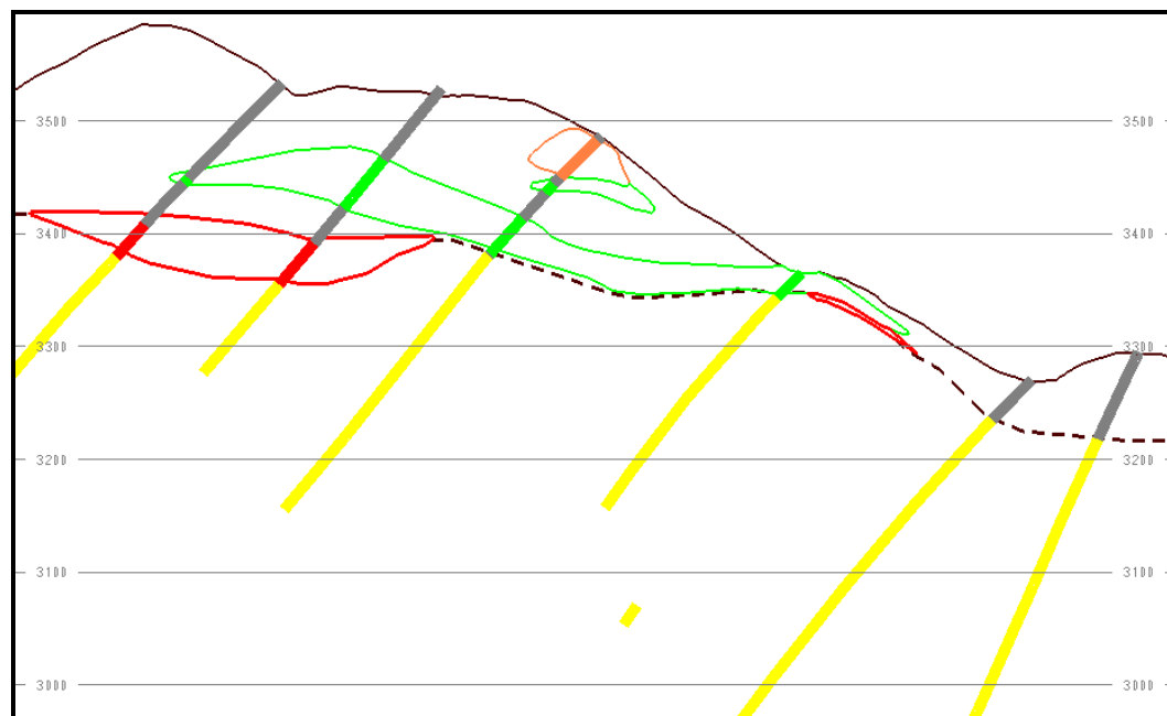
Figure 7.4 Diagram of Porphyry-Style Mineralization Zonation
