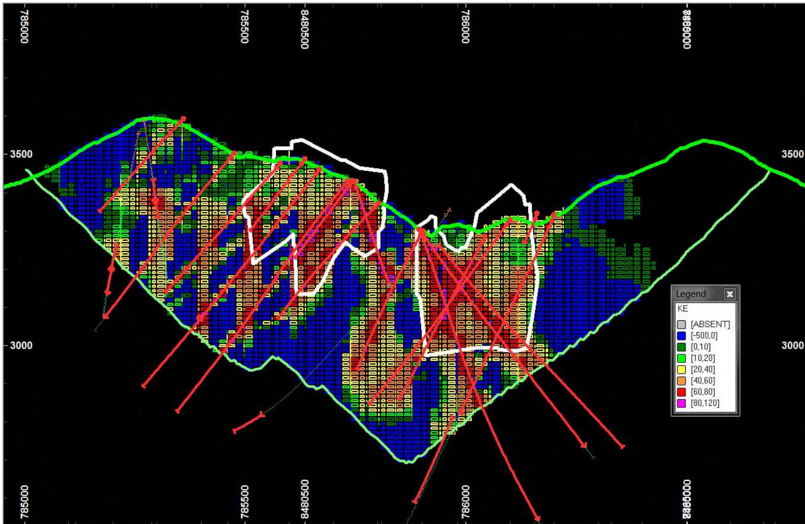
Figure 14.32 Resource Indicated Classification Wireframe (White) within Conceptual Pit Shell
