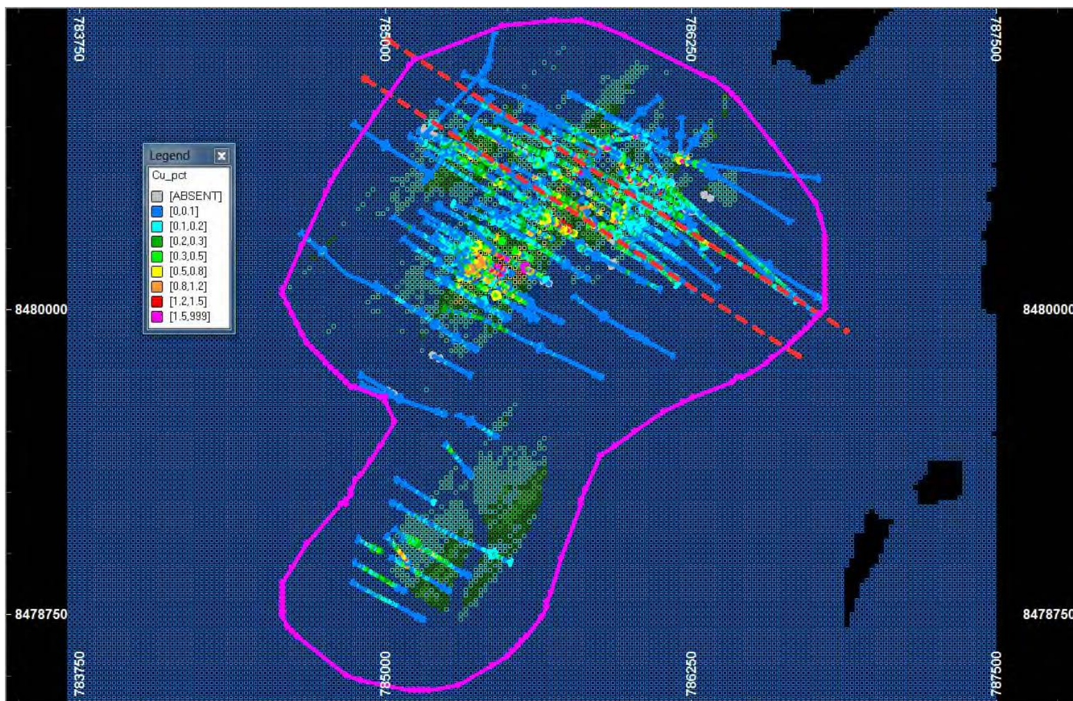
Figure 14.13 Plan View (3,200 m elevation) Showing Conceptual Pit Outline (magenta) and Northwest-Southeast (red dashed lines)
