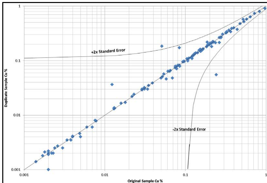
Figure 12.3 Reject Duplicate Control Graph
