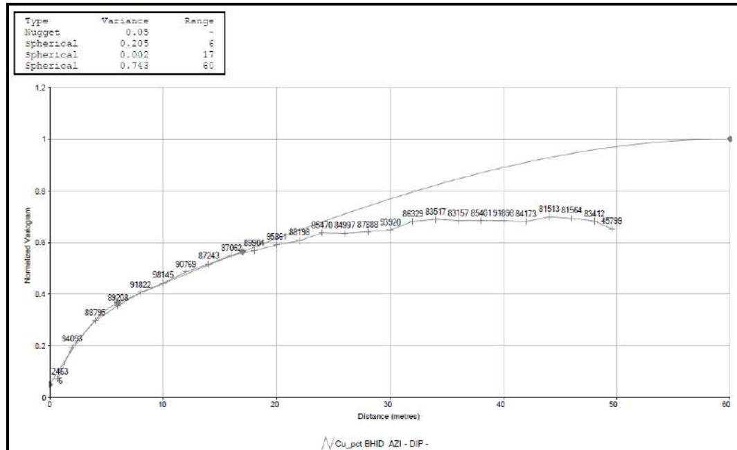
Figure 14.7 Copper Downhole Variograms for Zone 1 (Hypogene Mineralization)
