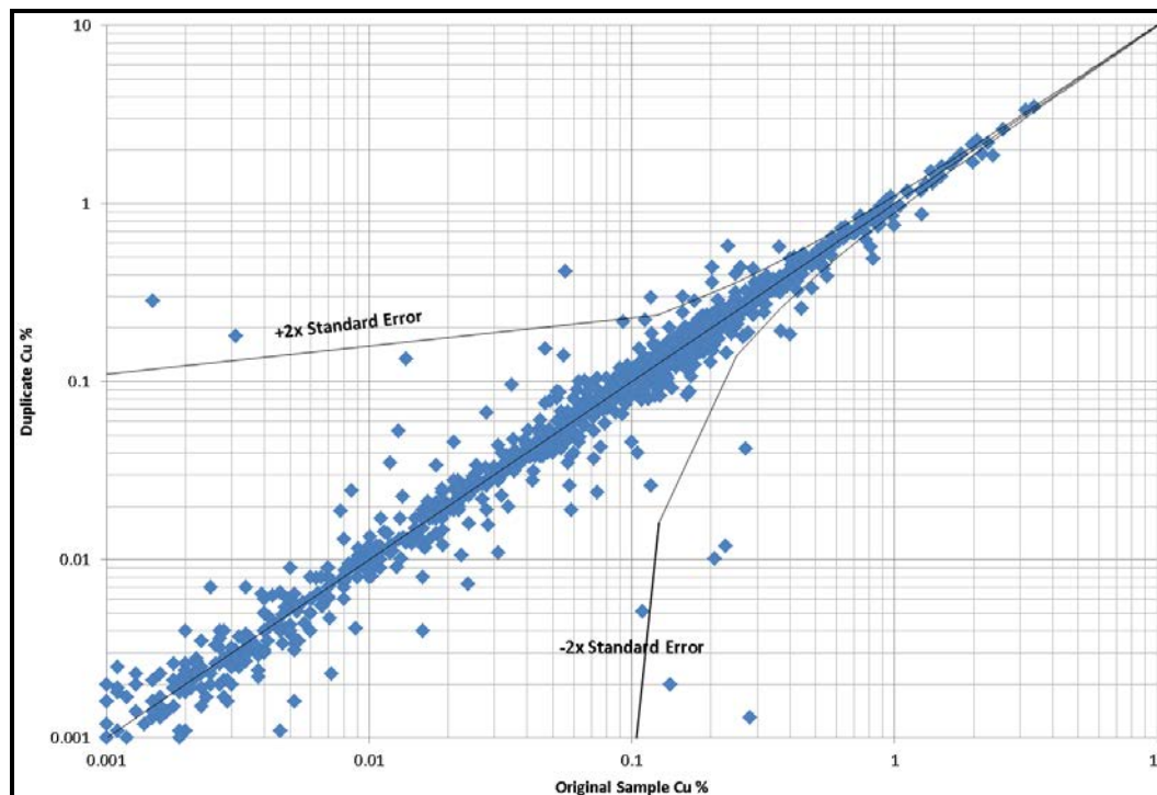
Figure 12.4 Pulp Duplicate Control Graph
