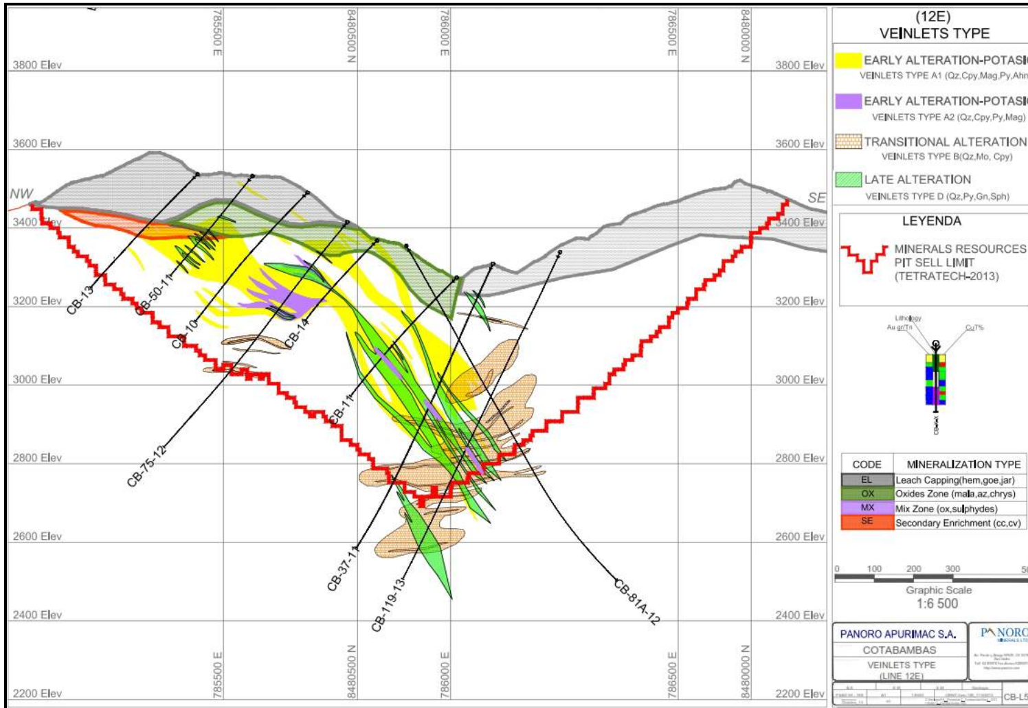
Figure 7.5 Typical Cross-section of Porphyry-Style Mineralization Zonation in Cotabambas
