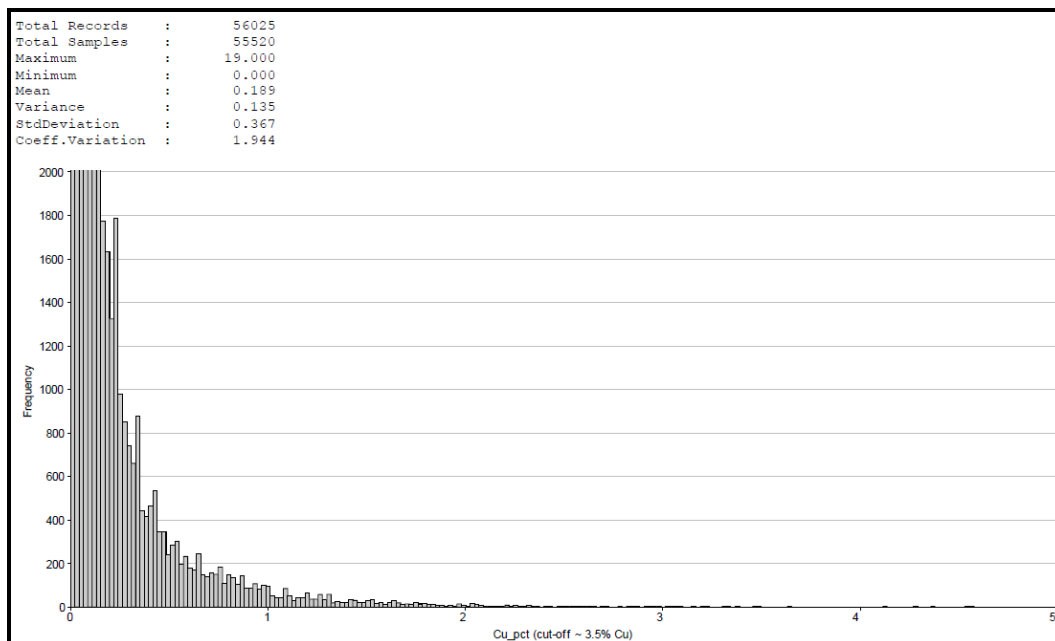
Figure 14.3 Copper Log Histogram of Raw Drillhole Data
