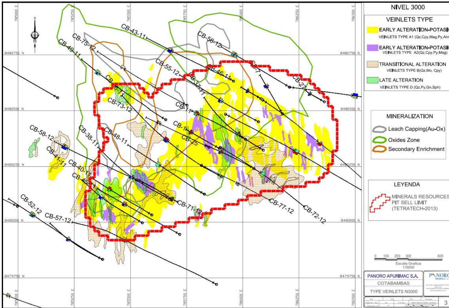
Figure 7.6 Plan View of Level 3000 of the Porphyry-Style Mineralization Zonation in Cotabambas
