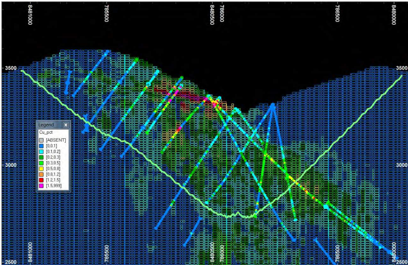
Figure 14.14 Copper Northwest-Southeast Section Furthest to Northeast Showing Cu %
