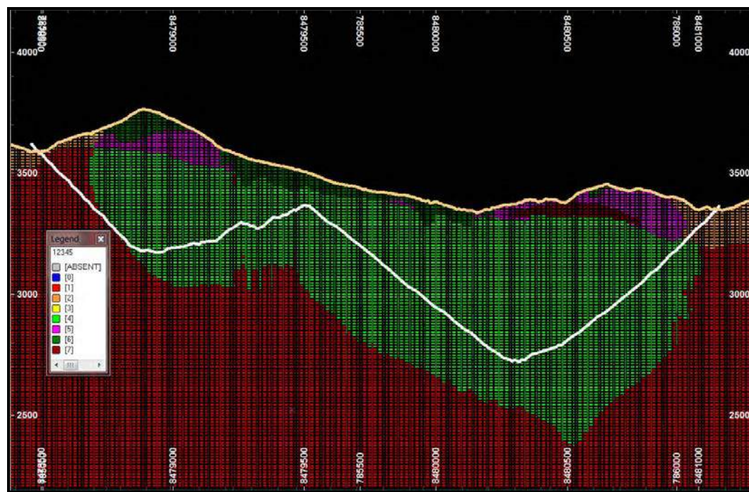
Figure 14.34 Conceptual Pit Shell Cross-section (south-southwest to north-northeast)
