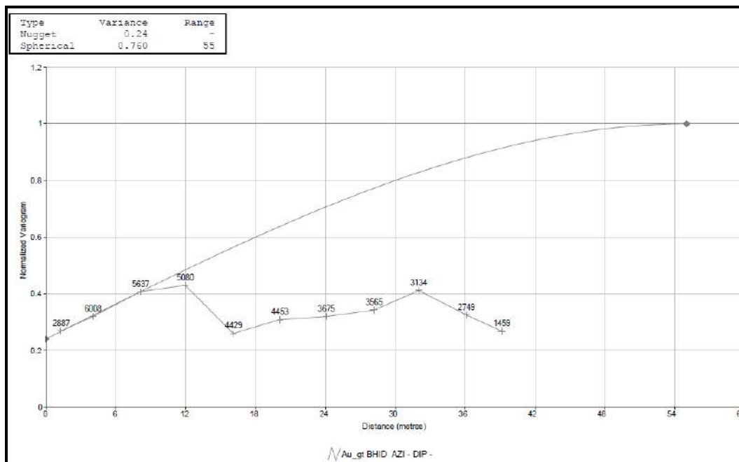
Figure 14.9 Gold Downhole Variograms for Zone 2 (Oxide Mineralization)
