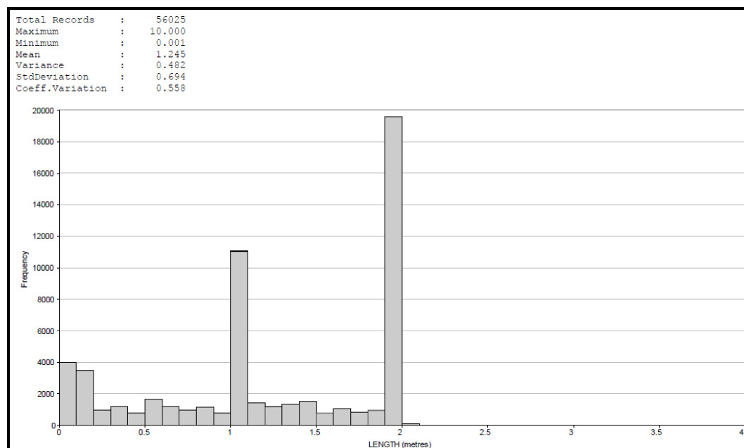
Figure 14.6 Sample Length Histogram of Raw Drillhole Data
