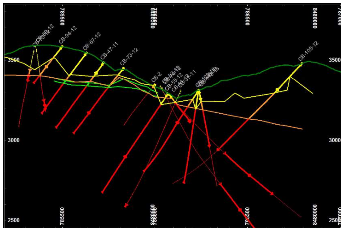
Figure 14.1 Northwest-southeast Cross-section of Domain Wireframes with Drillhole Traces, Coloured by Domain (yellow – leached cap, orange – oxide, bright green – supergene, red – hypogene)
