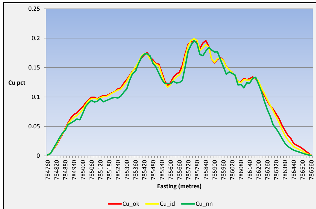
Figure 14.24 Copper Swath Plot by Easting (metres)
