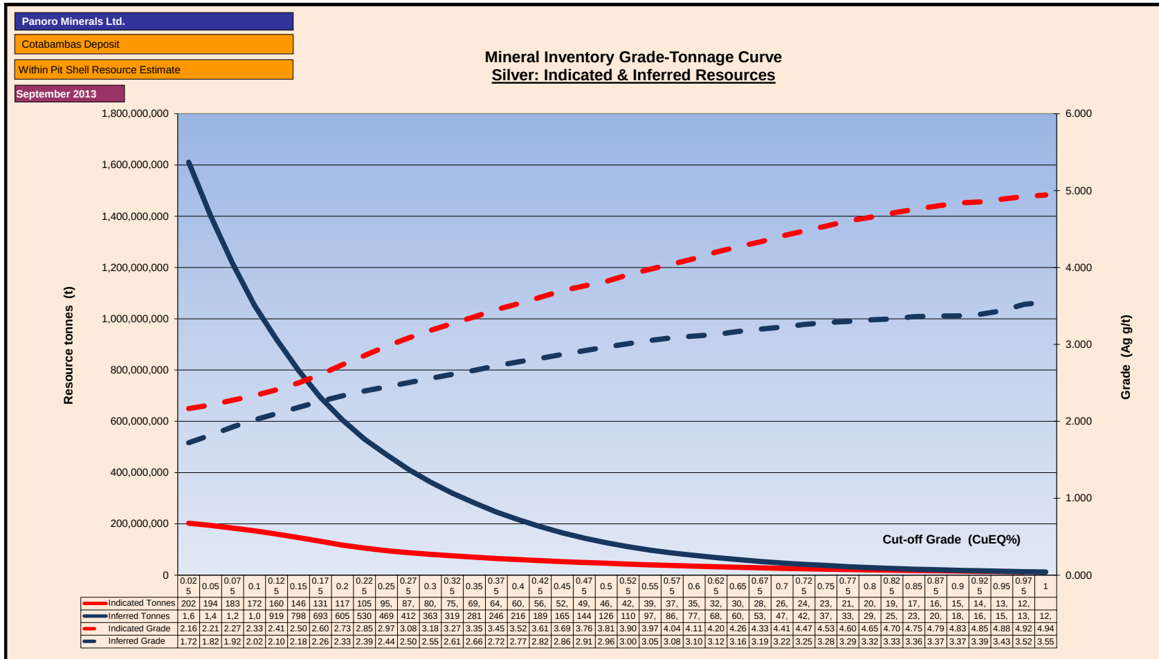
Figure 14.37 Indicated and Inferred Resources Silver Grade-Tonnage Curve
