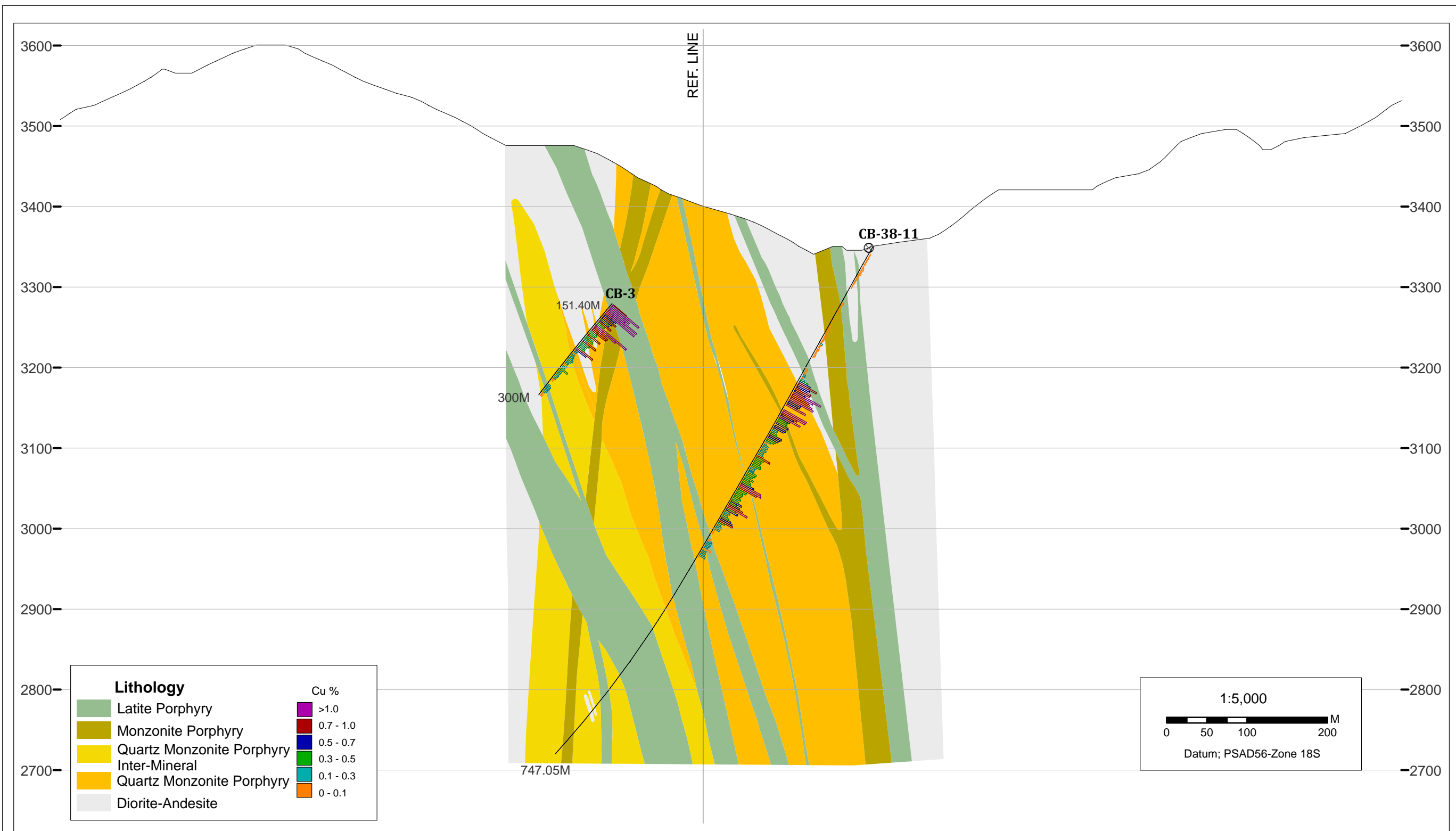
Geologic Section 08E COTABAMBAS PROJECT - APURIMAC PERU
