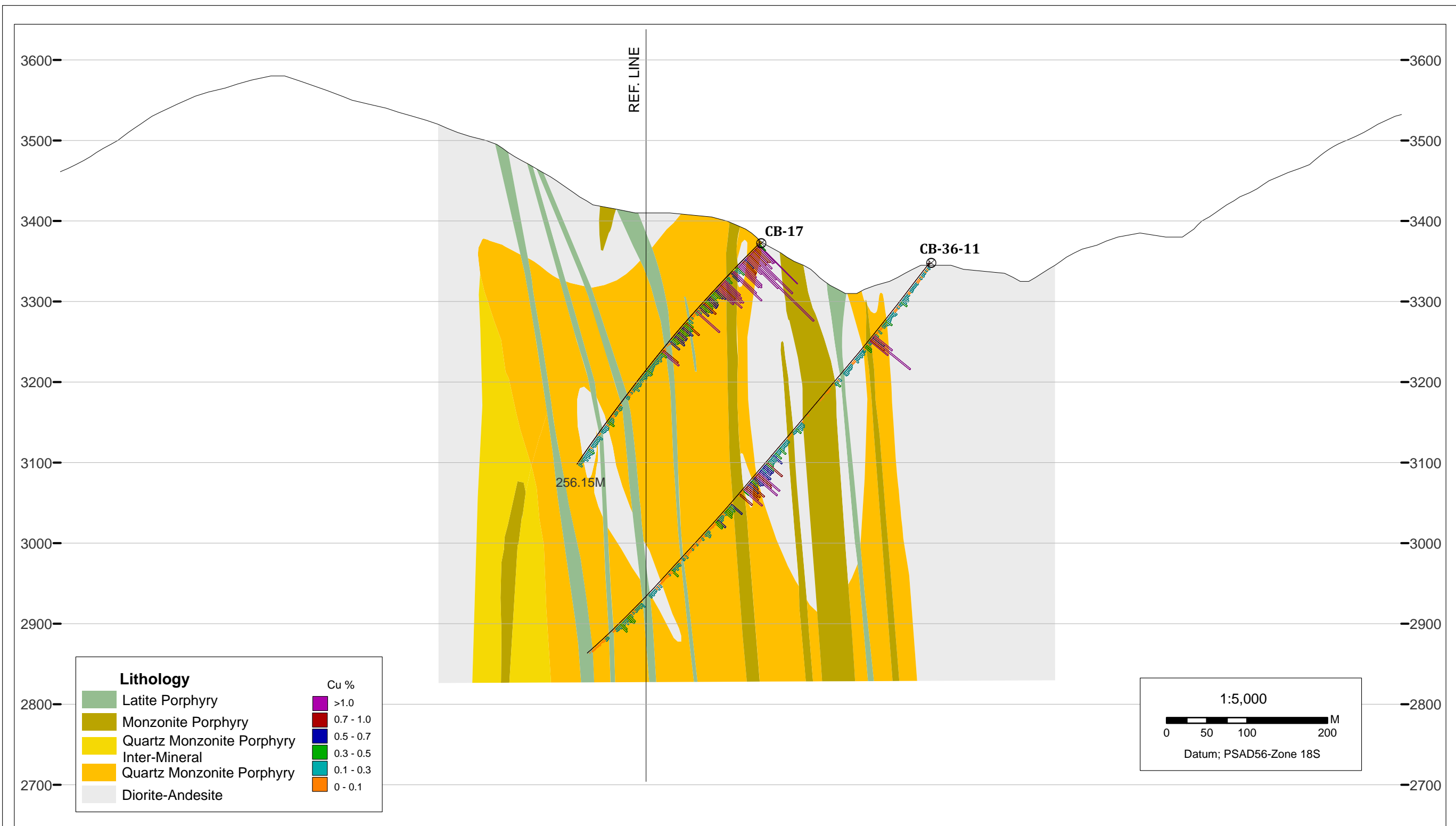
Geologic Section 10E COTABAMBAS PROJECT - APURIMAC PERU
